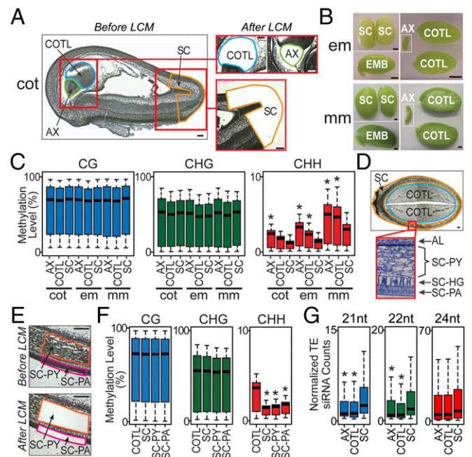
Fig. 3. Comparison of methylomes between soybean seed parts and SC layers. (A) Paraffin sections of cot-stage SC, embryonic AX, and embryonic COTL before and after capture by LCM. (B) Whole-mount pictures of SC, AX, and COTL from em- and mm-stage EMB and seeds. (C) Box plots of DNA methylation levels in 500-kb windows across the genome in different seed parts. Asterisks indicate significant comparisons between SC and other seed parts at the same stage ( t test, P < 0.001 and fold change > 1.5 ). (D) Paraffin cross-section of an em-stage seed (Upper), and a plastic section of SC layers (Lower), which is the red boxed region shown in the whole-seed section. (E) Paraffin cross-sections of em-stage SC-PA and SC-PY layers before and after capture by LCM. (F) Box plots of LCM-captured em-stage COTL, SC, SC-PA, and SC-PY DNA methylation levels in 500-kb windows across the genome. Asterisks indicate significant comparisons between SC, SC layers, and the COTL ( t test, P < 0.001 and fold change > 1.5 ). (G) Box plots of TE siRNA levels (reads per million mapped reads) in em-stage SC, AX, and COTL. Asterisks indicate statistically significant comparisons between SC and other seed parts ( t test, P < 0.001 and fold change > 1.5 ). [Scale bars, 100 \mu m (A, D, and E) and 1 mm (B).] See Table 1 for abbreviations.
